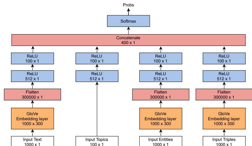
Figure 3. A deep learning architecture for the classification of news-feeds using raw text, topics, named entities, and triples.
