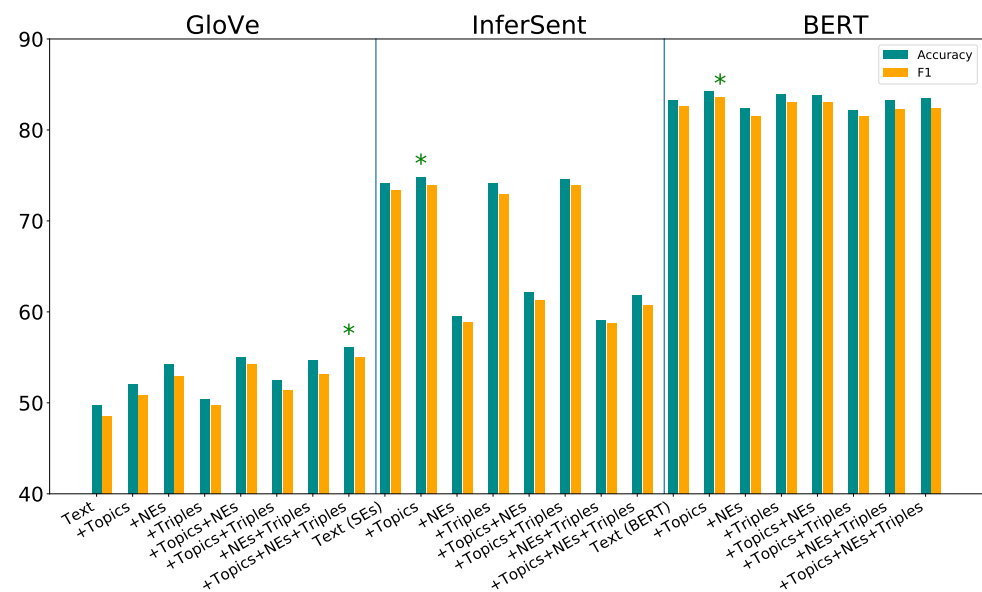
Figure 8. Performance results of classifiers from different inputs on the 20 News groups dataset. The first block of results uses GloVe-based representations. The second block is models using the InferSent sentence encoder. The third block uses BERT-based models. * indicate the best model from each class.
